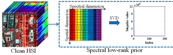
Fig. 3. Spectral low-rank prior of the clean HSI.
