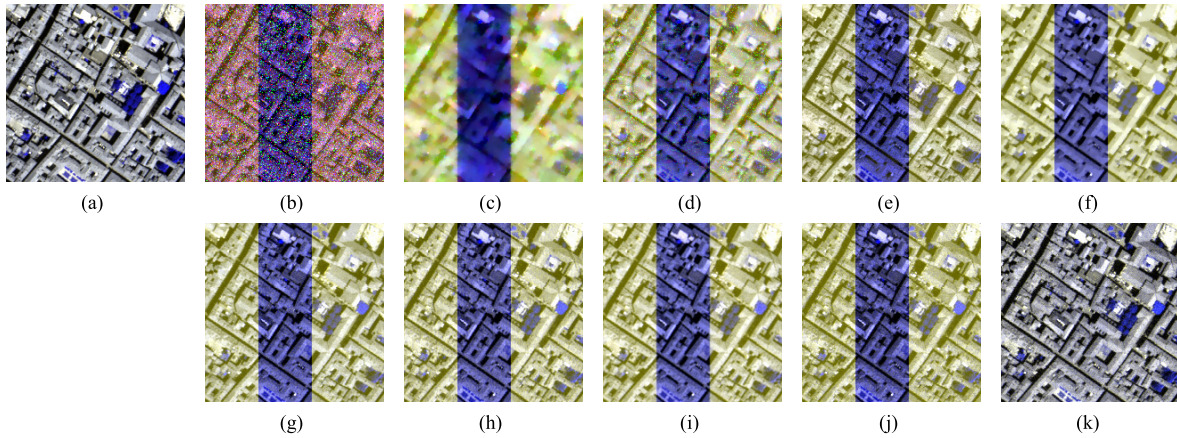
Fig. 12. Simulation experiment denoising false-color results in case 6. (a) Original image (R: 27, G: 31, B: 53). (b) noisy image (12.32 dB). (c) SSAHTV (19.09 dB). (d) BM4D (20.38 dB). (e) LRM (23.46 dB). (f) LRTV (22.94 dB). (g) LLRSSTV (24.02 dB). (h) LRTDGS (23.81 dB). (i) 3-DLogTNN (24.01 dB). (j) LRTDFDR (22.75 dB). (k) DLR (34.73 dB).
