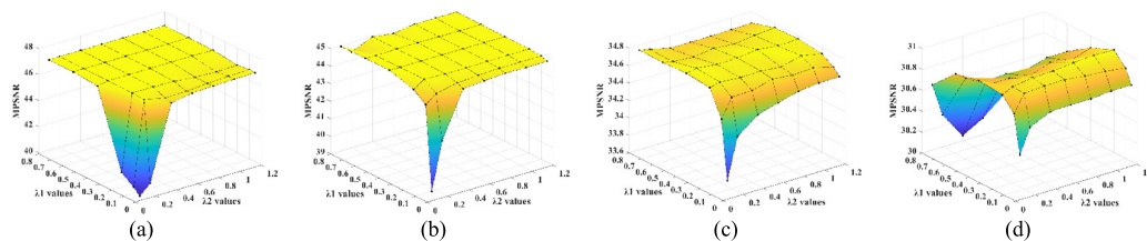
Fig. 20. Change in the MPSNR values of DLR in simulated case 1, with respect to parameters \lambda_1 and \lambda_2 . (a) V = 0.001 , P = 0.05 . (b) V = 0.01 , P = 0.1 . (c) V = 0.05 , P = 0.15 . (d) V = 0.1 , P = 0.2 .
