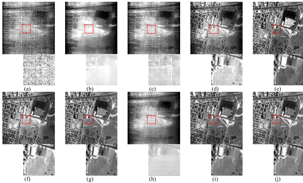
Fig. 13. Denoising results for band 107 of the HYDICE Urban data set via the different methods. (a) Original image. The denoised images of (b) SSAHTV, (c) BM4D, (d) LRM, (e) LRTV, (f) LLRSSTV, (g) LRTDGS, (h) 3-DLogTNN, (i) LRTDFDR, and (j) DLR.
