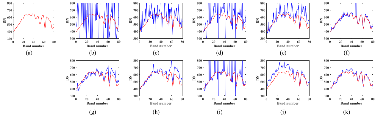
Fig. 8. Original spectrum (red curve) and the denoising results (blue curve) of pixel (193.68) in simulated case 4. (a) Original. (b) Noisy. (c) SSAHTV. (d) BM4D. (e) LRM. (f) LRTV. (g) LRSSTV. (h) LRTDGS. (i) 3-DLogTNN. (j) LRTDFDR. (k) DLR.
