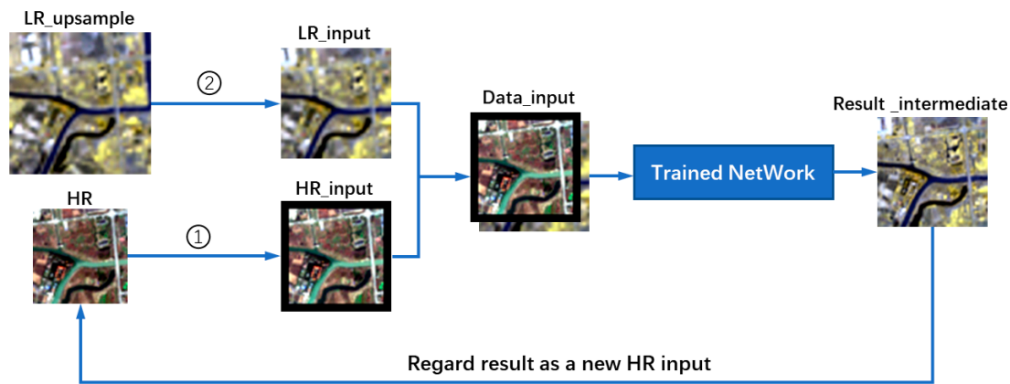
Figure 3. The process of the recurrent expanding strategy. Step 1: Expand the high spatial resolution (HR) data by several pixels assigned to 0. Step 2: Crop the low spatial resolution (LR)_upsample data to the same size and same coverage as the HR_input.
